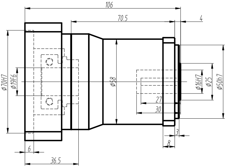
标准轴 Standard output shaft
