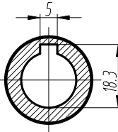
标准轴 Standard output shaft
